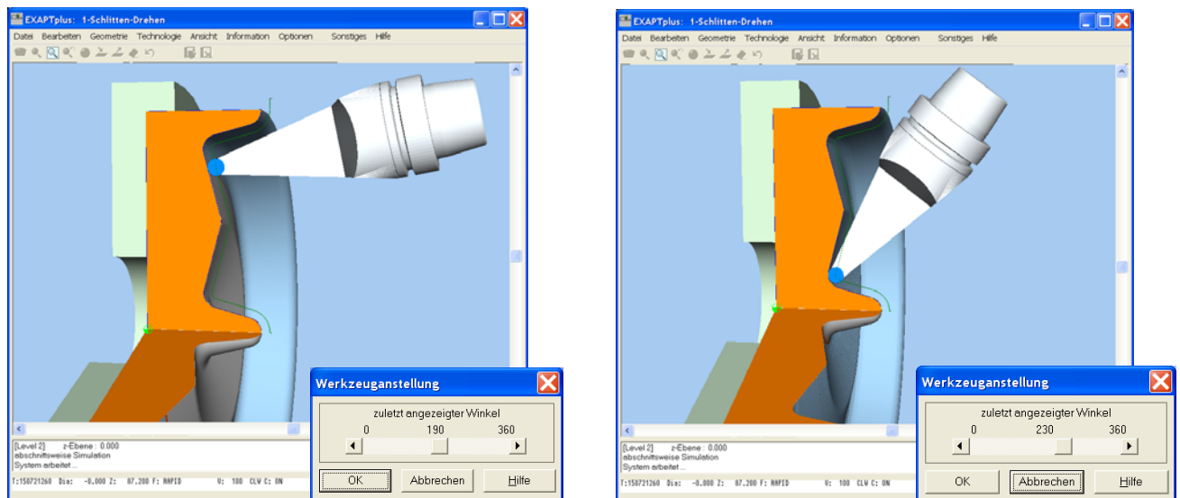
Fig.: Simulation B-axis turning
